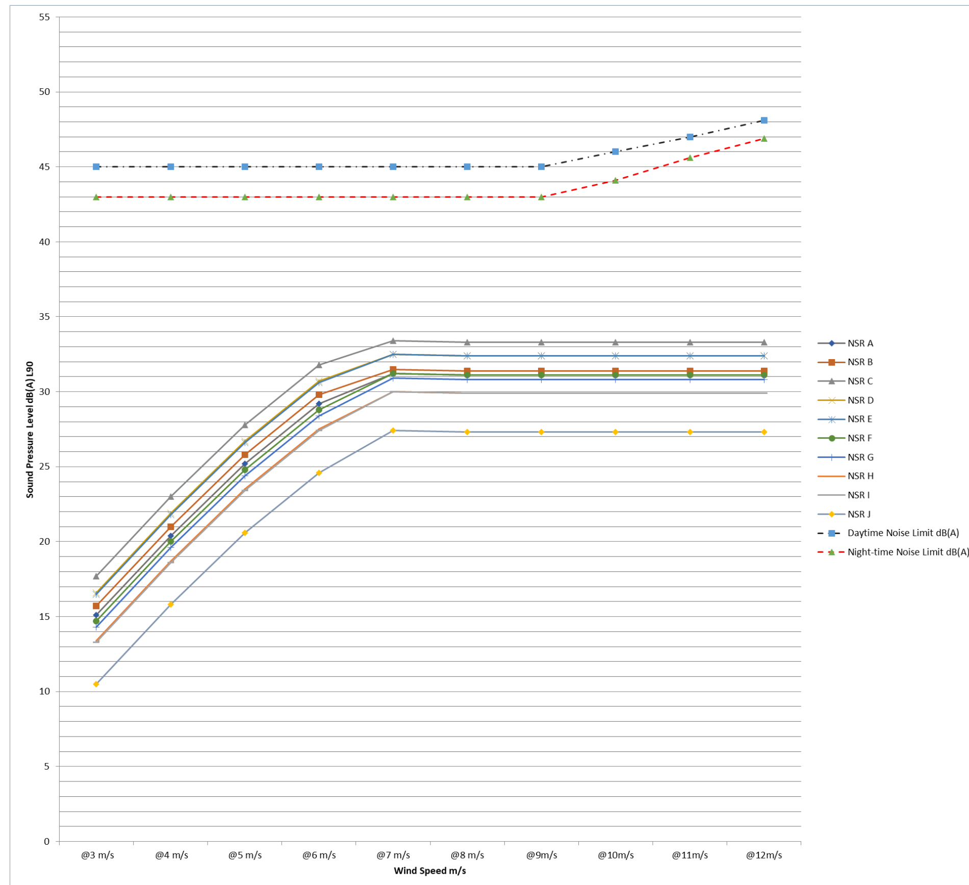
Figure 8.4 Predicted L_{A90} windfarm noise levels at each of the noise assessment locations as a function of standardised wind speed for the WTG Project Design Option 1 (Model 1B) from the Array Area, versus the WEDG2006 Guidelines noise limit
