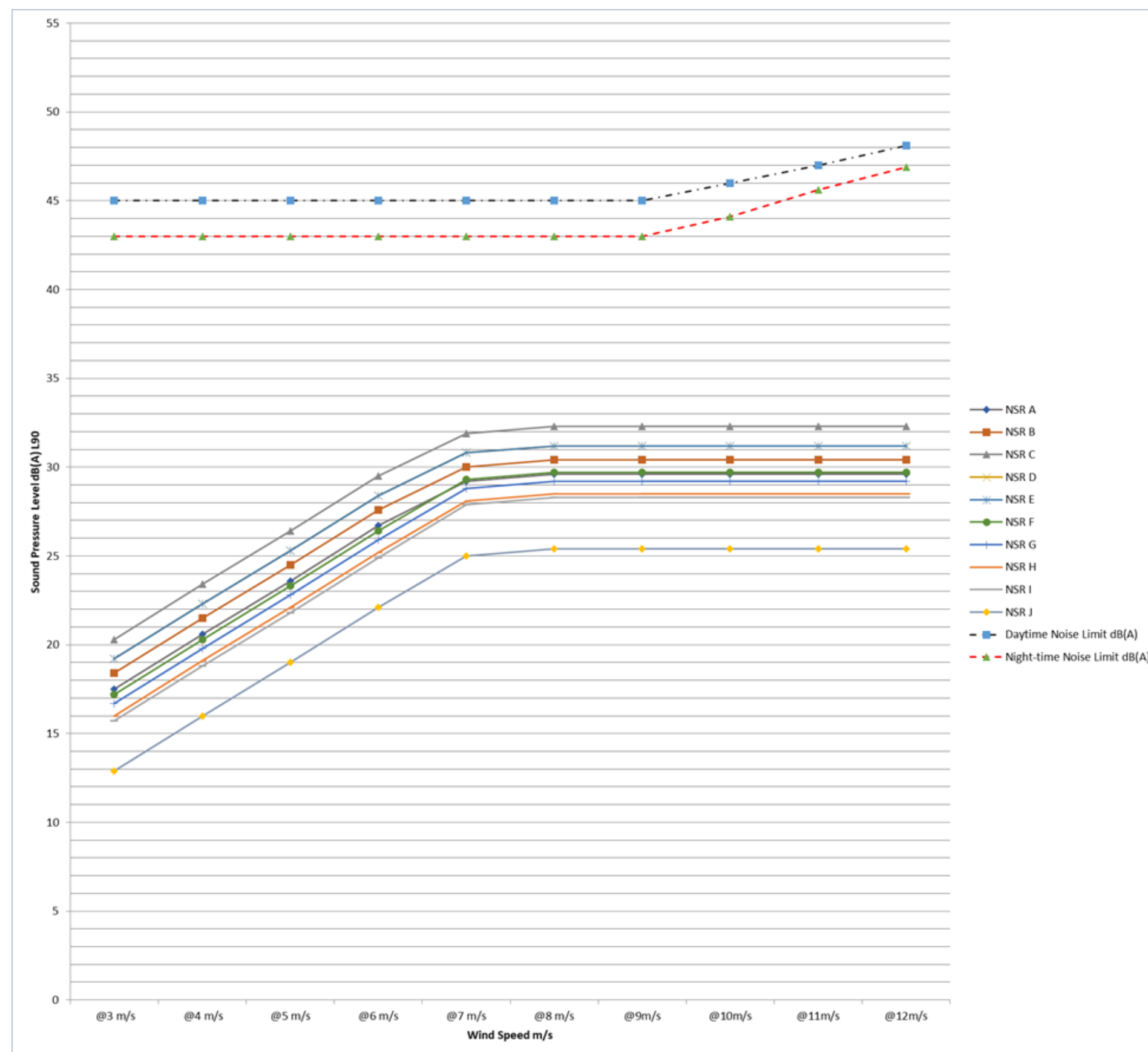
Figure 8.6: Predicted L_{A90} windfarm noise levels at each of the noise assessment locations as a function of standardised wind speed for WTG Project Design Option 2 from the Array Area, versus the 2006 Guidelines noise limit
