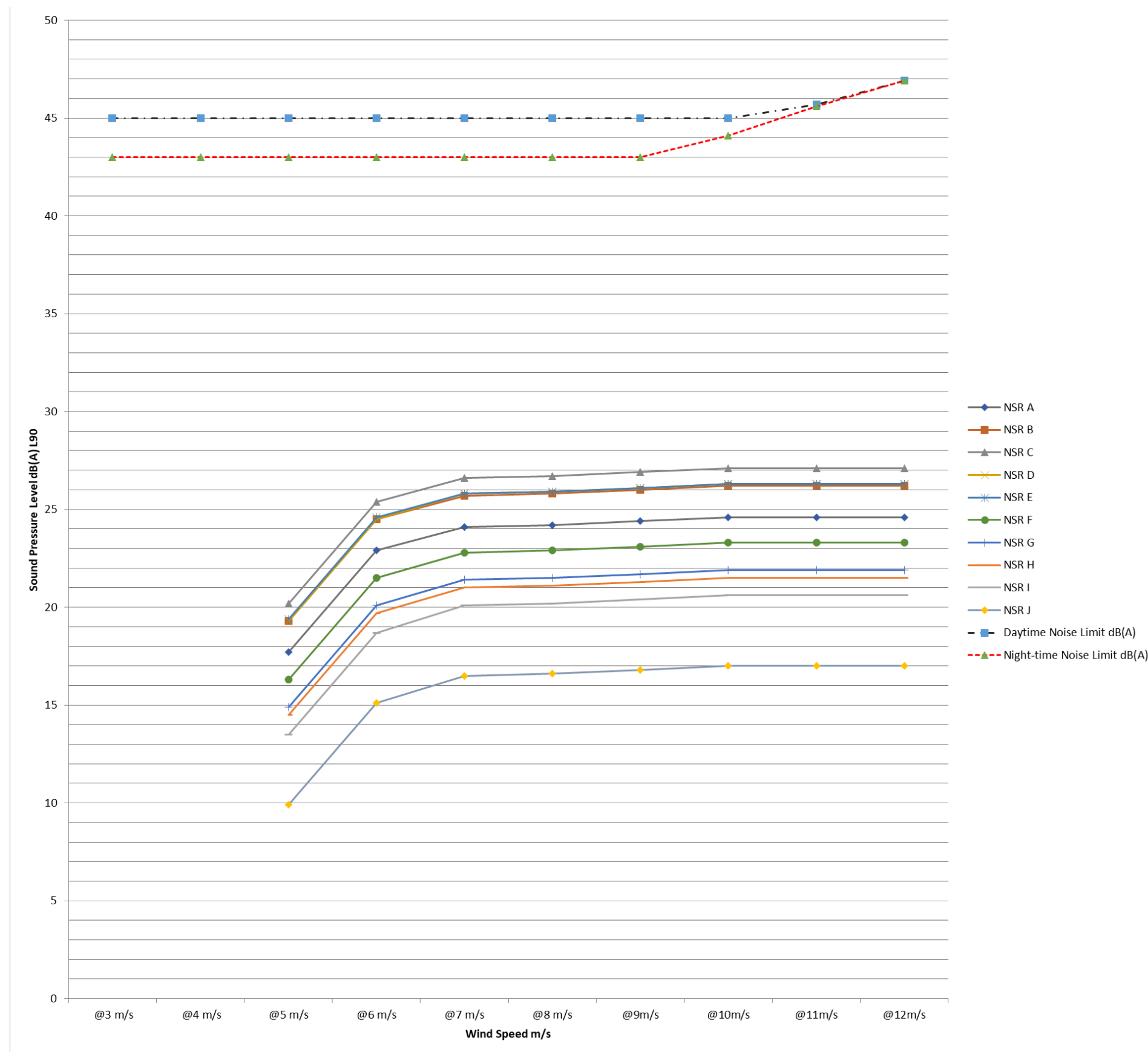
Figure 8.3 Predicted LA90 windfarm noise levels at each of the noise assessment locations as a function of standardised wind speed for the WTG Project Design Option 1 (Model 1A) from the Array Area, versus the WEDG2006 Guidelines noise limit
