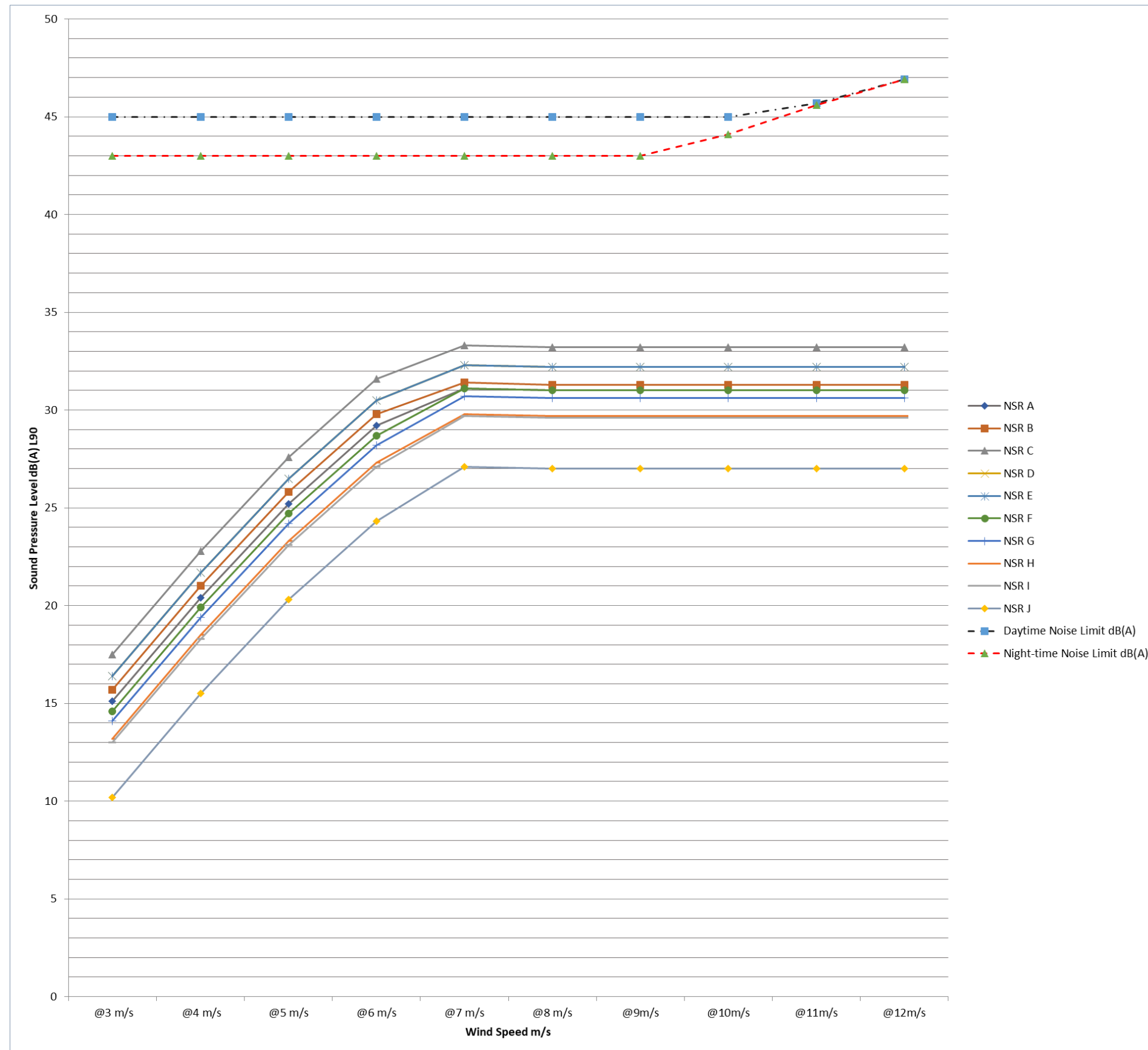
Figure 8.5 Predicted \text{L}_{A90} windfarm noise levels at each of the noise assessment locations as a function of standardised wind speed for the WTG Project Design Option 1 (Model 1B) from the Array Area, versus the WEDG2006 Guidelines noise limit
